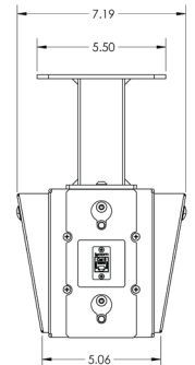
Ceiling Mount Side
