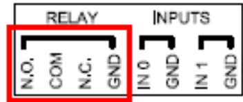
Board Connections
